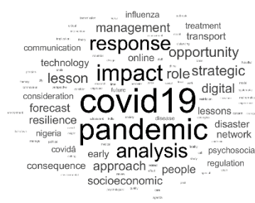
Topic: 2
