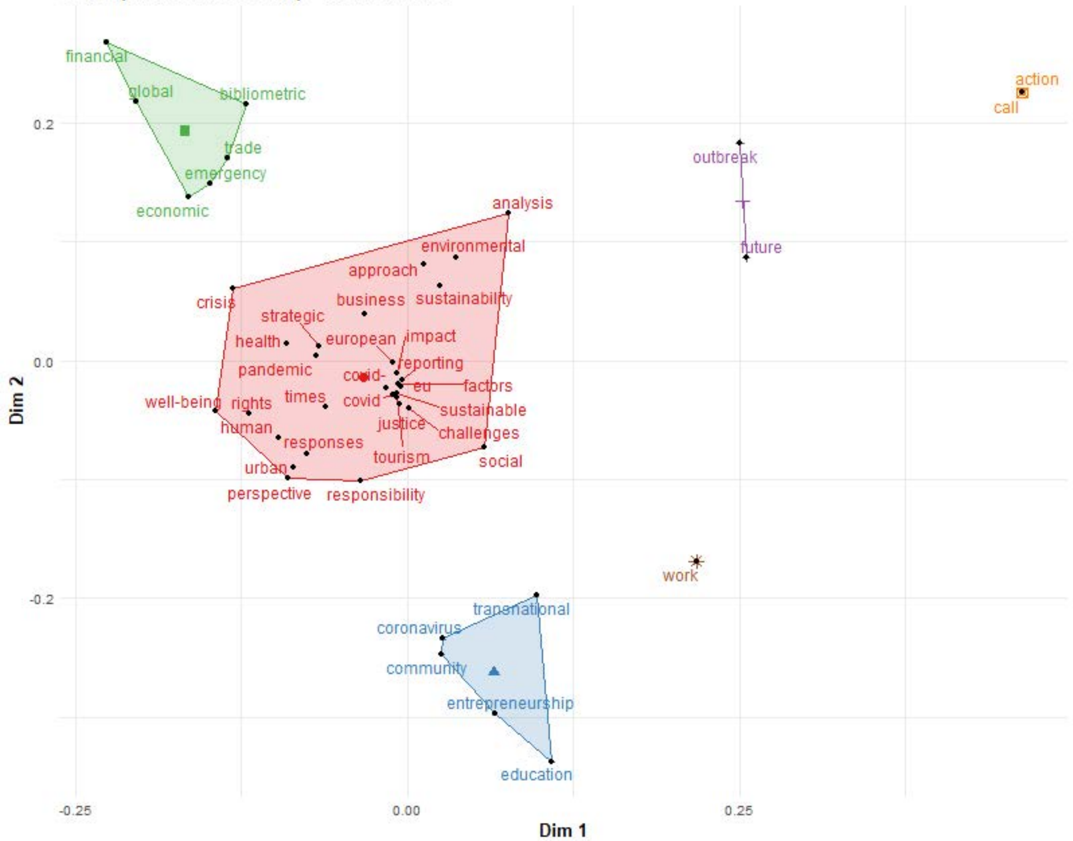
Conceptual Structure Map - method: MDS
