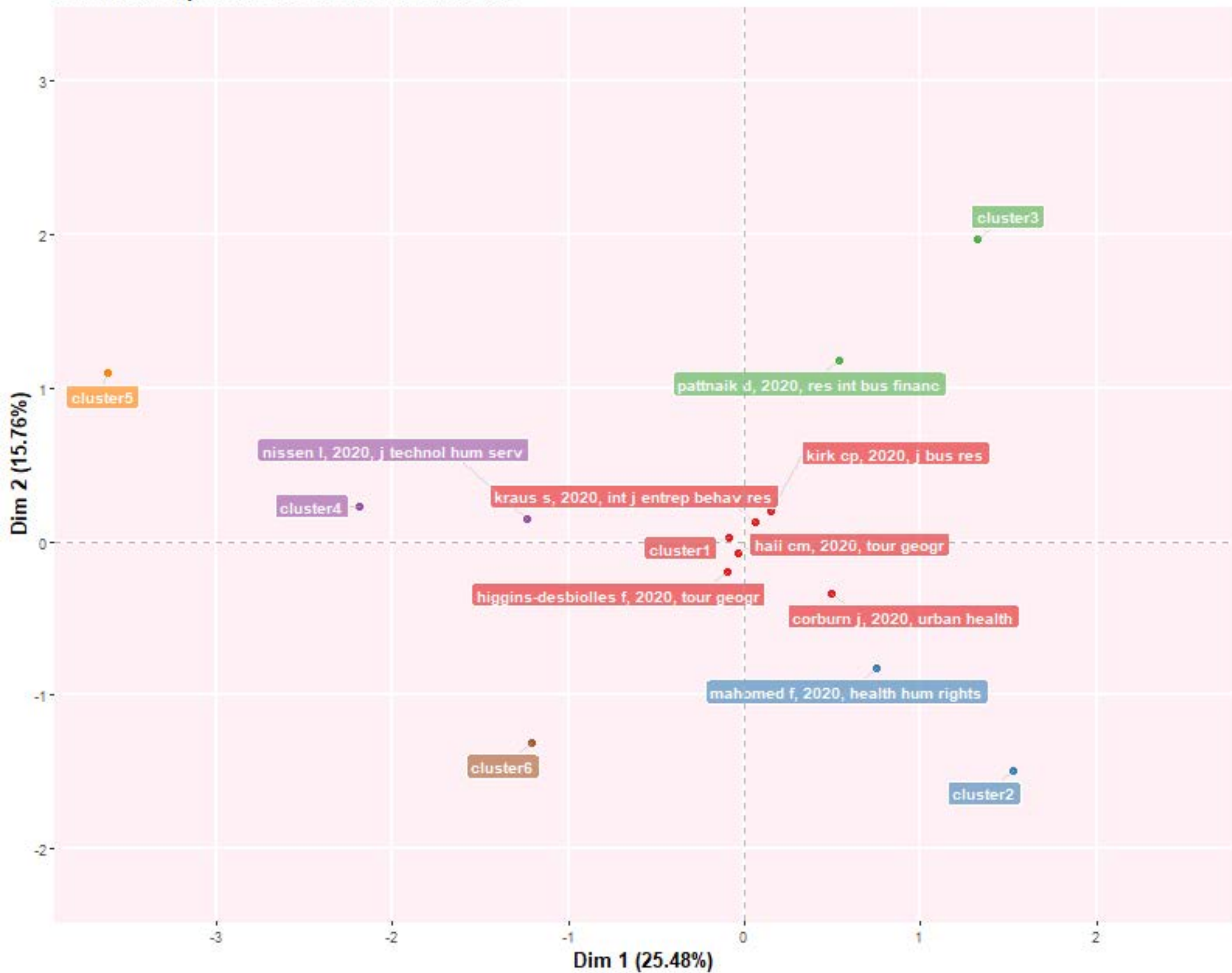
Factorial map of the most cited documents
