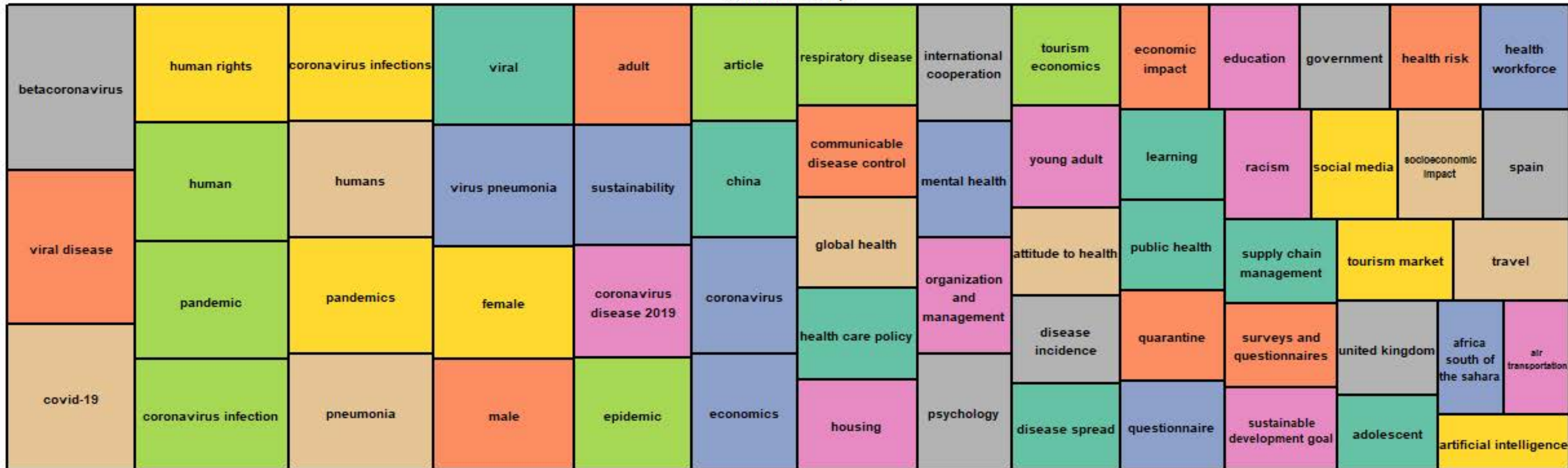
Word TreeMap
