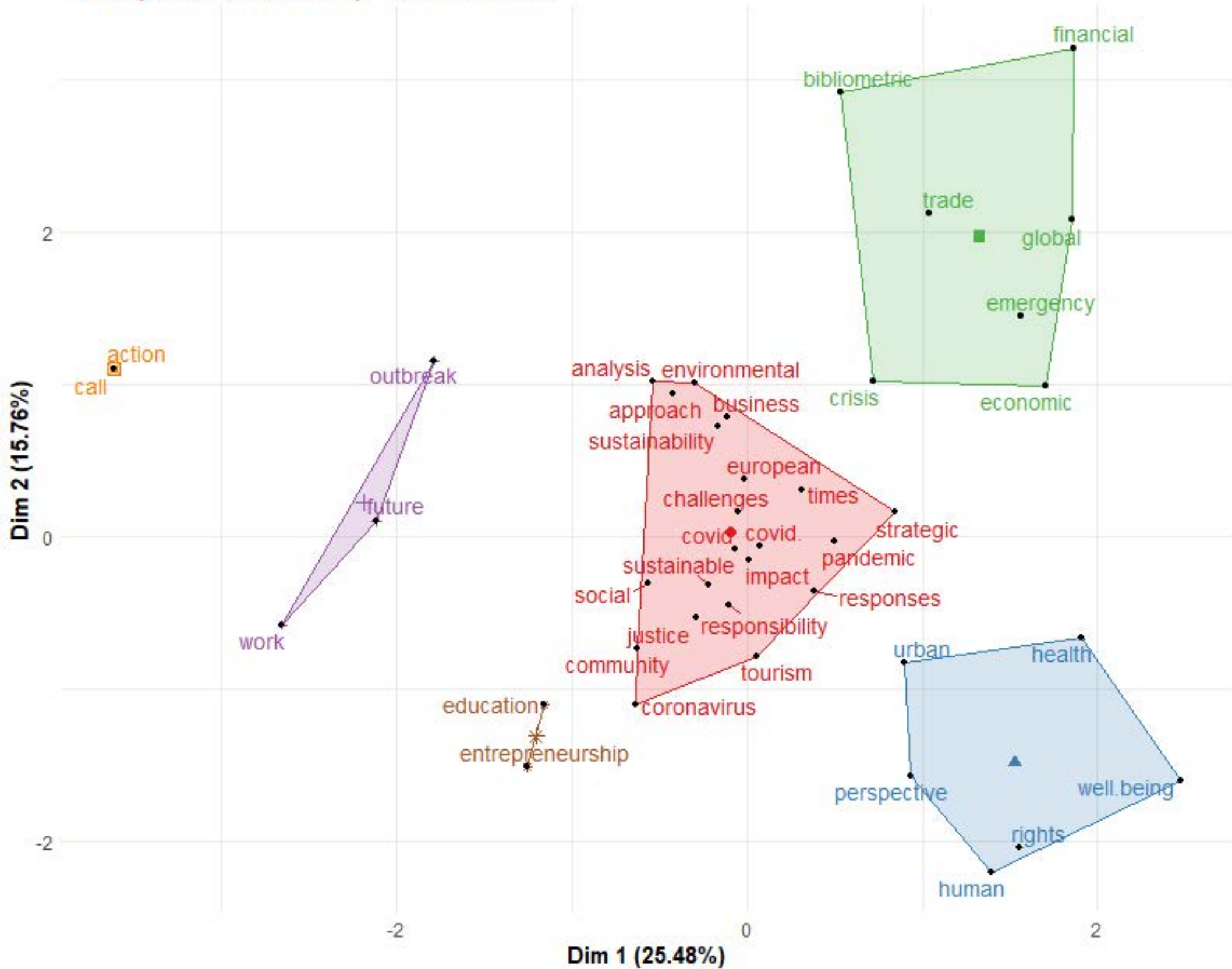
Conceptual Structure Map - method: MCA
