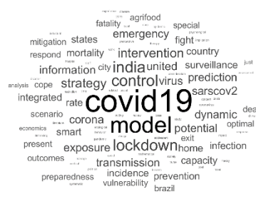
Topic: 4
