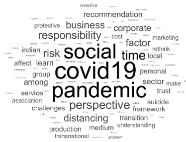
Topic: 1
