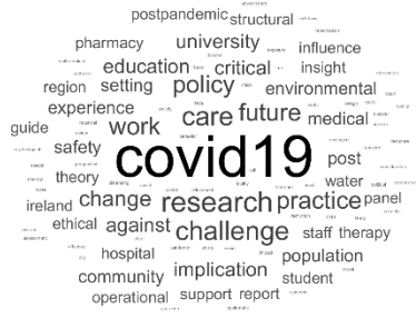
Topic: 3
